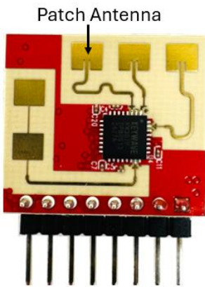
Front view (antenna facing forward)
